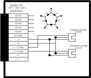
PHTM-60A105R接线图
