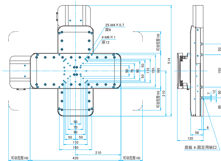
HST-200XY 内六角螺栓 M6×15...8个
