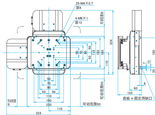
HST-100XY 内六角螺栓 M6×15...4个
